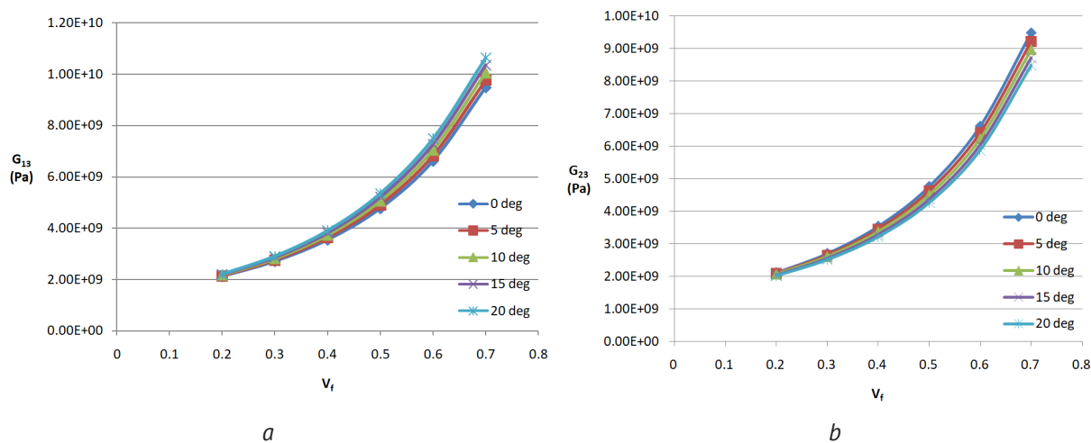
Figure 4 – (a) G_{13} vs V_f (b) G_{23} vs V_f
