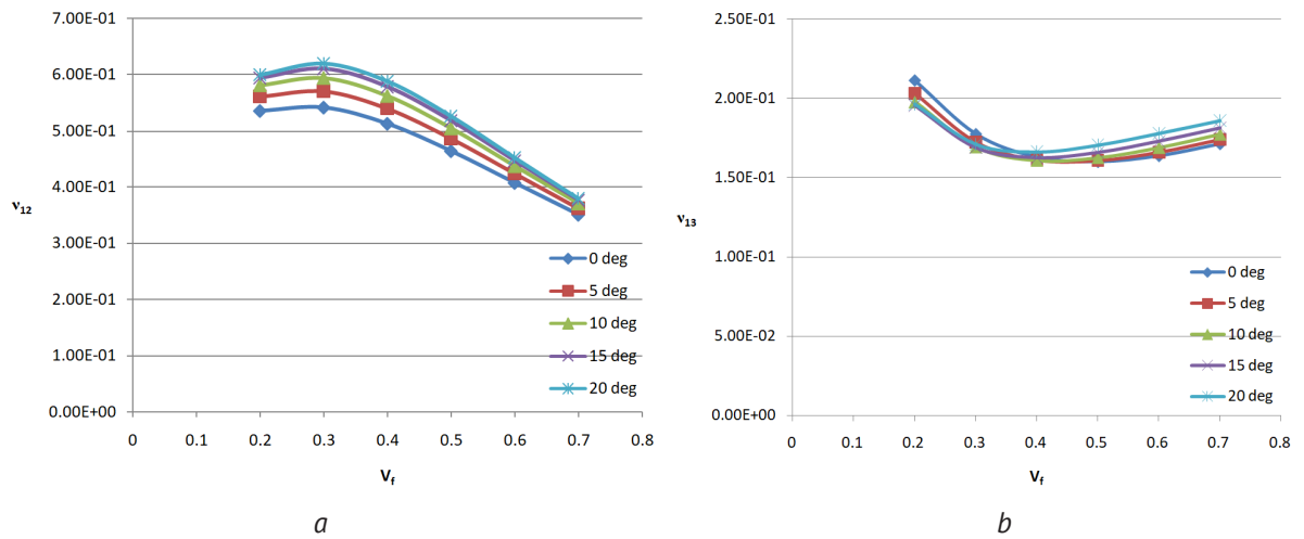
Figure 5 – (a) \nu_{12} vs V_f (b) \nu_{13} vs V_f
