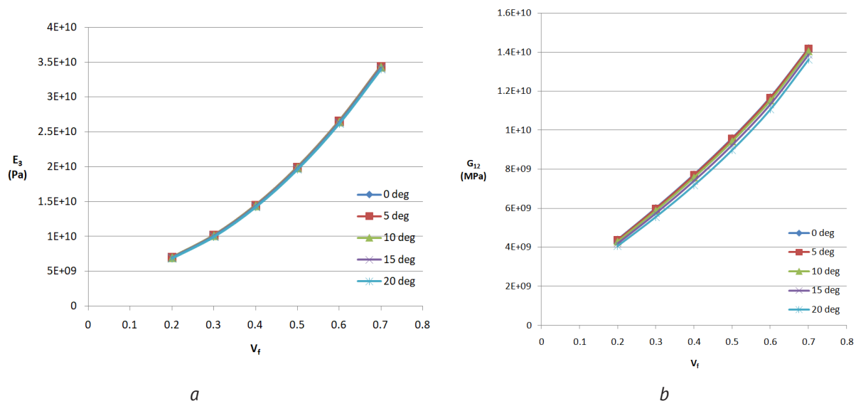
Figure 3 – (a) E_3 vs V_f (b) G_{12} vs V_f
