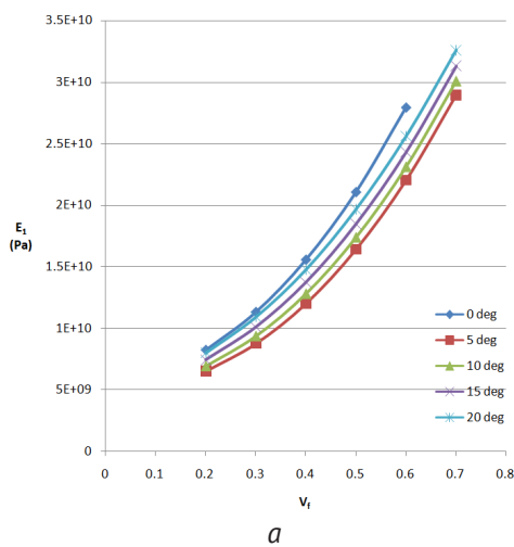
Figure 3 – (a) E_1 vs V_f (b) E_2 vs V_f
